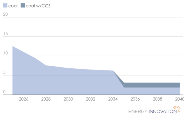
West Virginia Coal Generation Capacity, Jan. 2025 Forecast, GW
