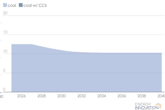
West Virginia Coal Generation Capacity, 2026 Forecast, GW
