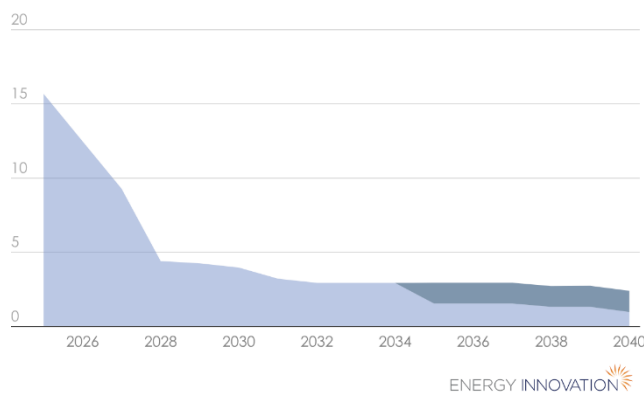
Texas Coal Generation Capacity, Jan. 2025 Forecast, GW
