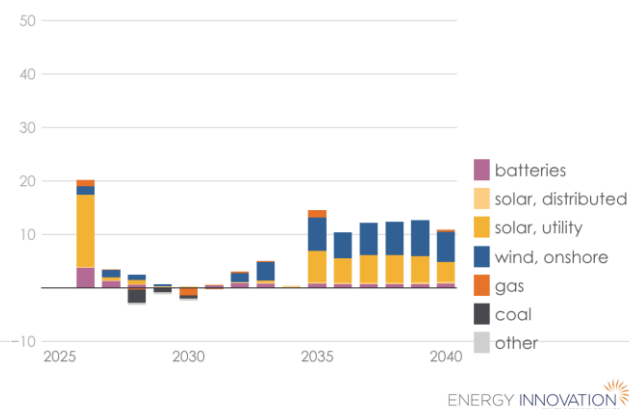
Net Annual Texas Electricity Capacity Additions, Retrofits, and Retirements
