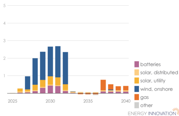
Net Annual Oregon Electricity Capacity Additions, Retrofits, and Retirements
