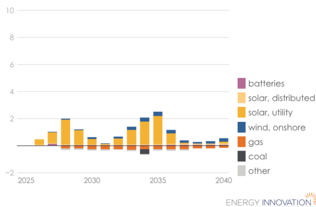
Net Annual North Carolina Electricity Capacity Additions, Retrofits, and Retirements
