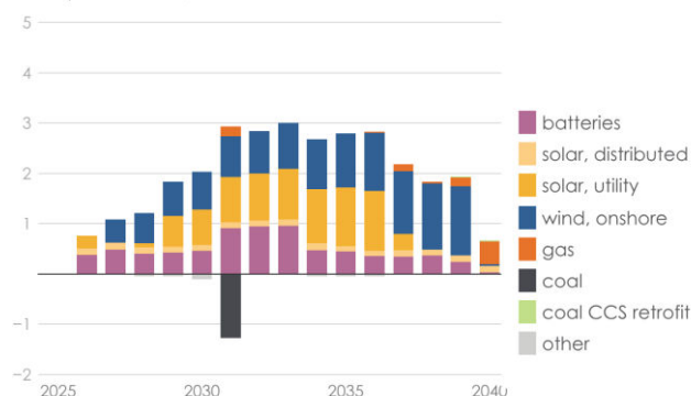
Net Annual Maryland Electricity Capacity Additions, Retrofits, and Retirements
