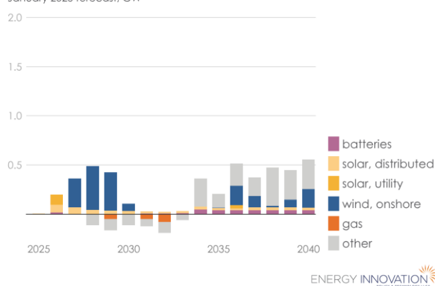
Net Annual Maine Electricity Capacity Additions, Retrofits, and Retirements
