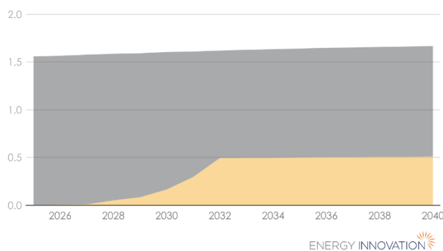
New Maine Freight HDV Sales, January 2025 Forecast
