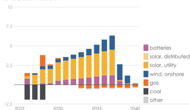
Net Annual Georgia Electricity Capacity Additions, Retrofits, and Retirements
