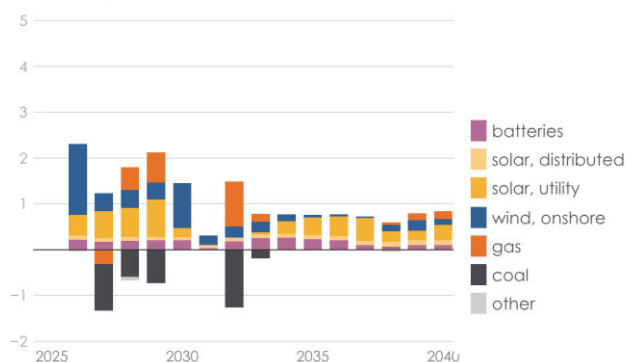
Net Annual Colorado Electricity Capacity Additions, Retrofits, and Retirements
