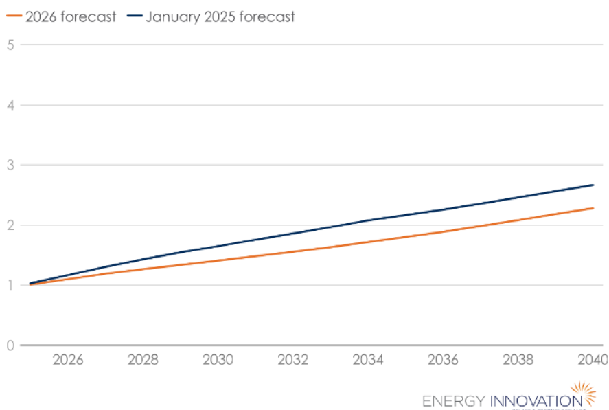
Colorado Distributed Solar Capacity, GW
