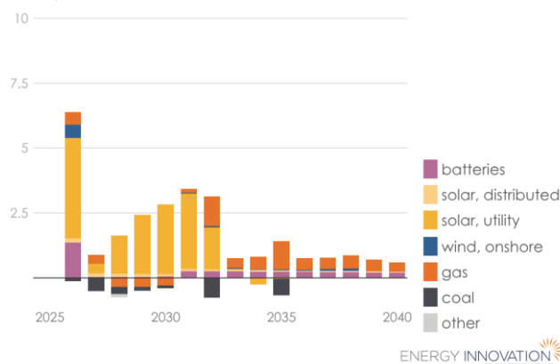
Net Annual Arizona Electricity Capacity Additions, Retrofits, and Retirements
