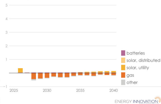
Net Annual Alabama Electricity Capacity Additions, Retrofits, and Retirements
