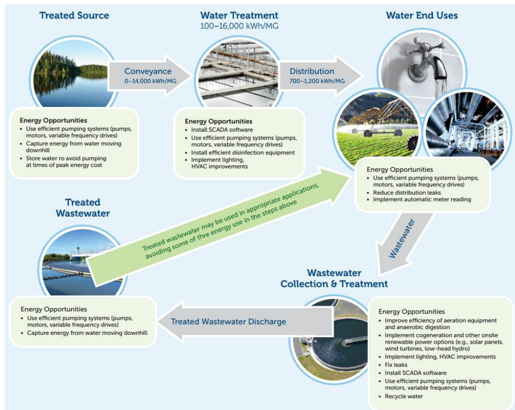
This graphic shows energy intensity of each stage in the water use cycle with key opportunities for energy efficiency, renewable energy, and water efficiency at each stage.
